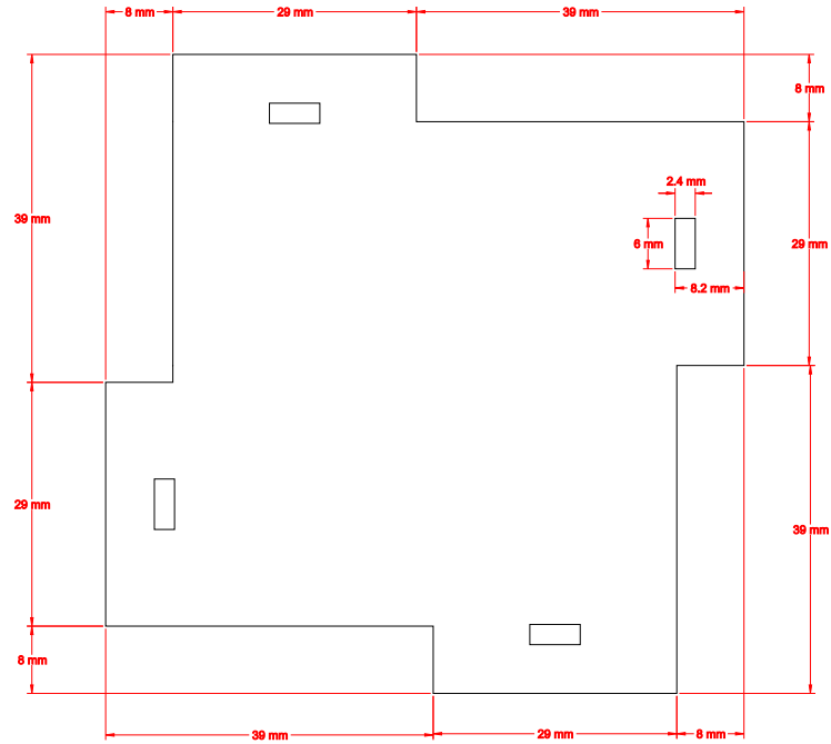
48pcs LASER CUT 2mm THK ES000 CLEAR ACRYLIC
